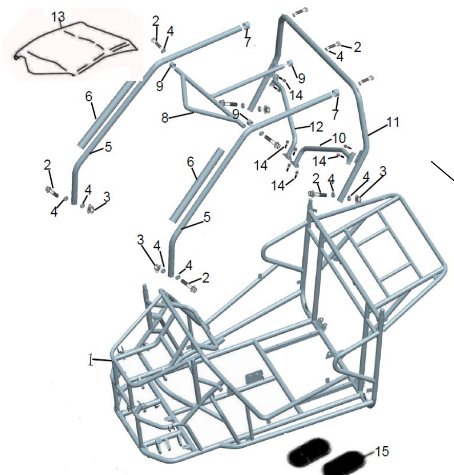
FIG. 1 FRAME GROUP
