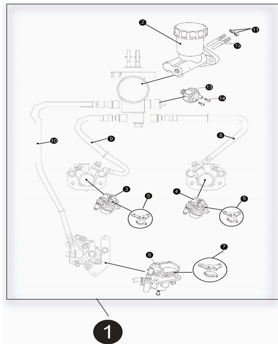
FIG. 22 BRAKE SYSTEM
