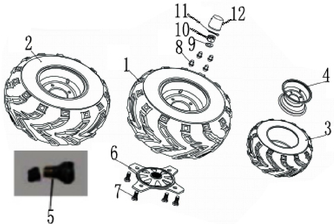
FIG. 20 REAR WHEEL
