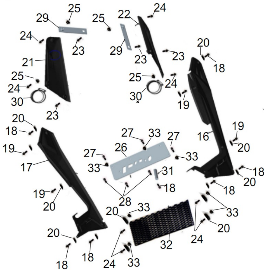
FIG. 24 Plastic parts 2
