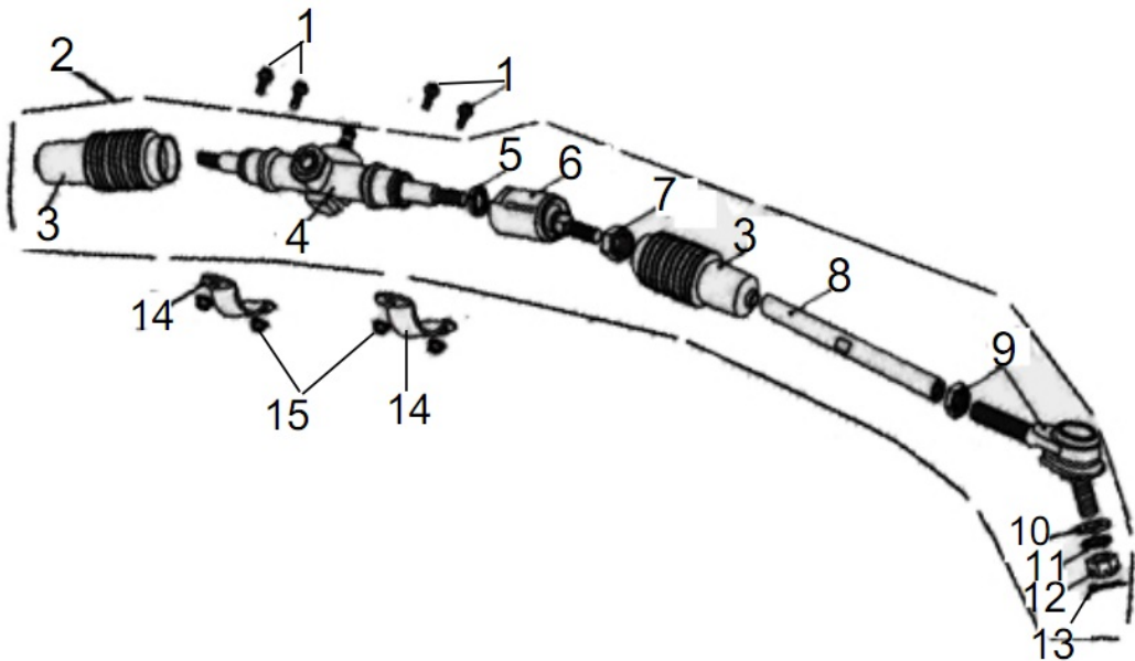
FIG. 6 STEERING GEAR ASSY.
