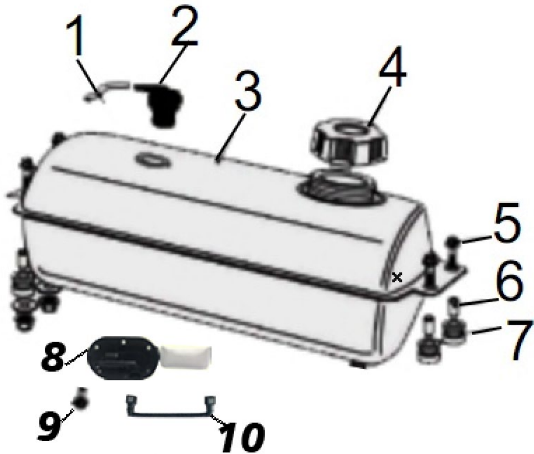
FIG. 11 FUEL TANK
