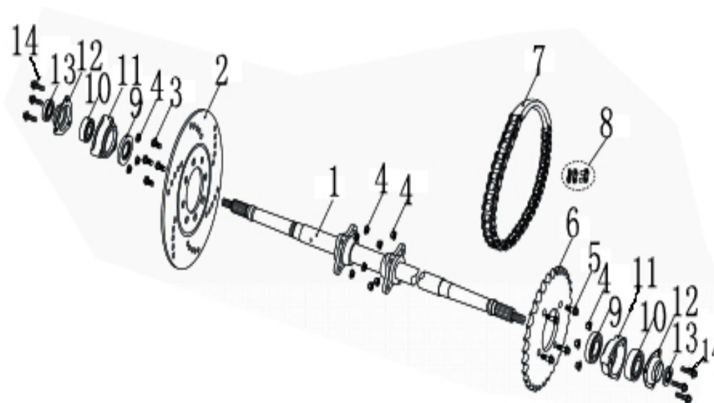
FIG. 21 REAR AXLE
